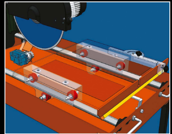
Working table sliding on six adjustable nylon wheels and twelve ball-bearings for higher precision and stability.
