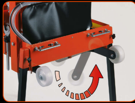
TRANSPORT WHEELS Folding wheels Ø 100 mm for a practical use
